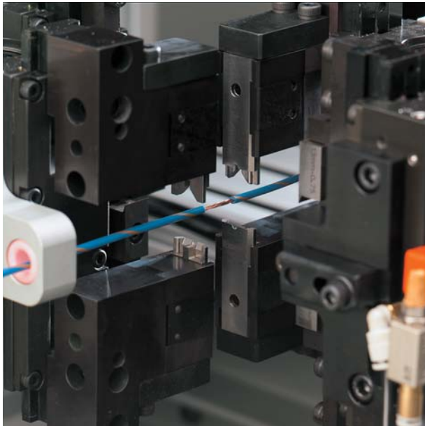
Mechtrix MX-5025 Center Stripping Machine
